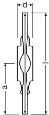
HQI-TS 70 W/NDL
