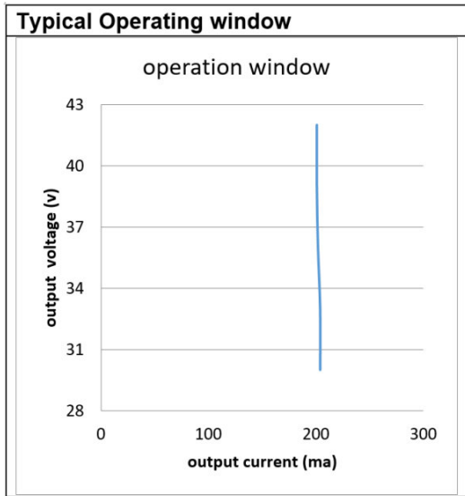
Operating Window
