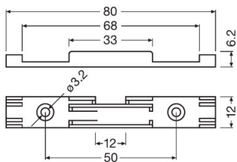
LR700SD-G1- PLATE FOR MAGNET
