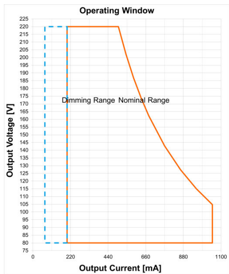
OT 110170-2401A0 1DIMLT2 G1 CE Operating Window
